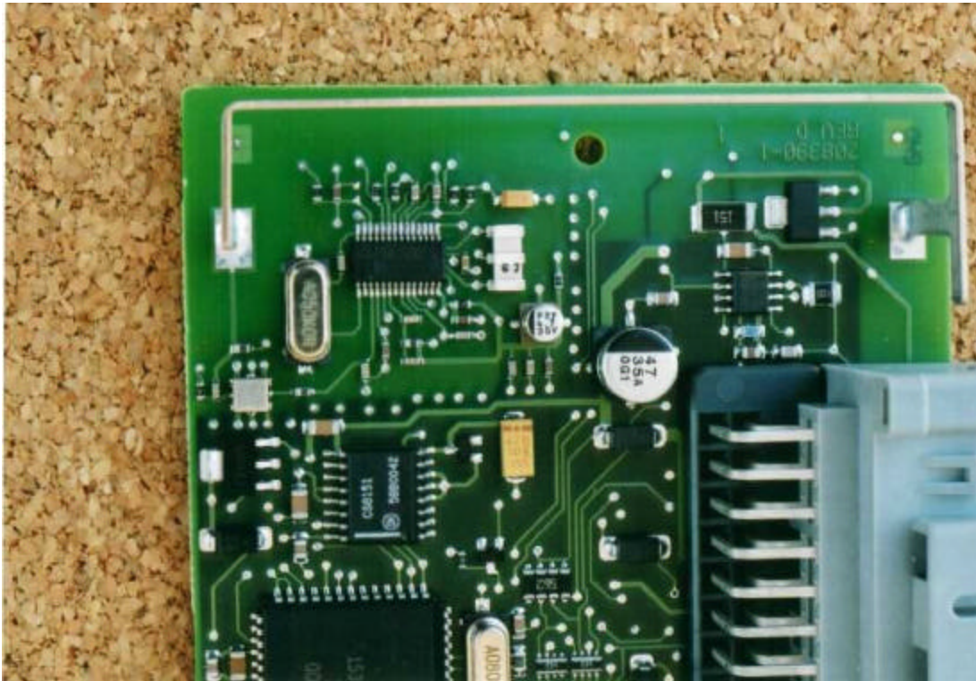
GQ43VT28R Receiver PCB RF Section Close-up Top
