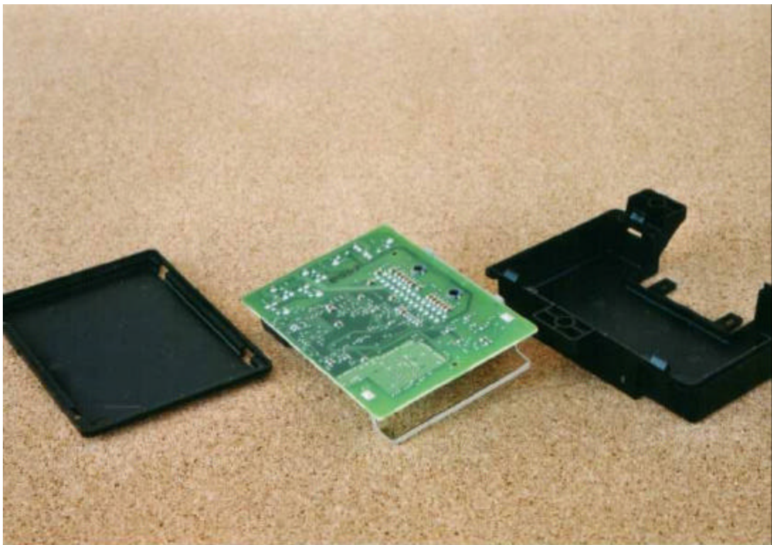
GQ43VT28R Receiver Open - Top
