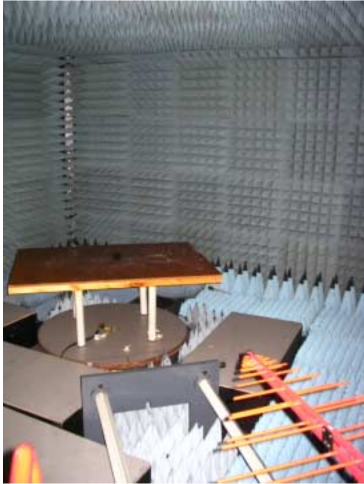
Photograph No.7 Setup for unintentional radiated emission measurements in anechoic chamber
