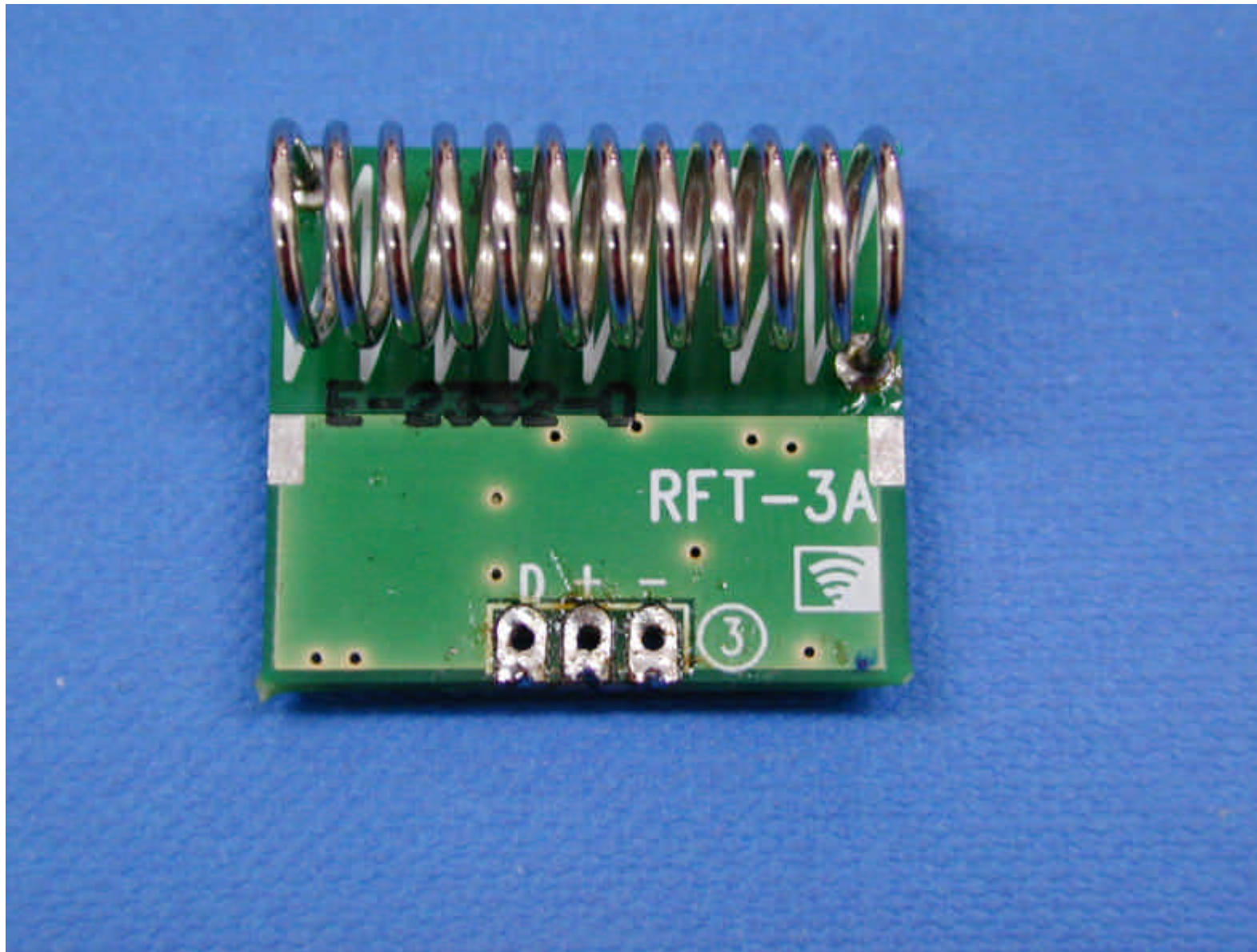
RF module first side
