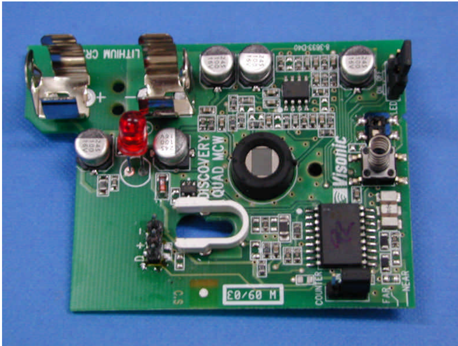
PCB first side without RF module
