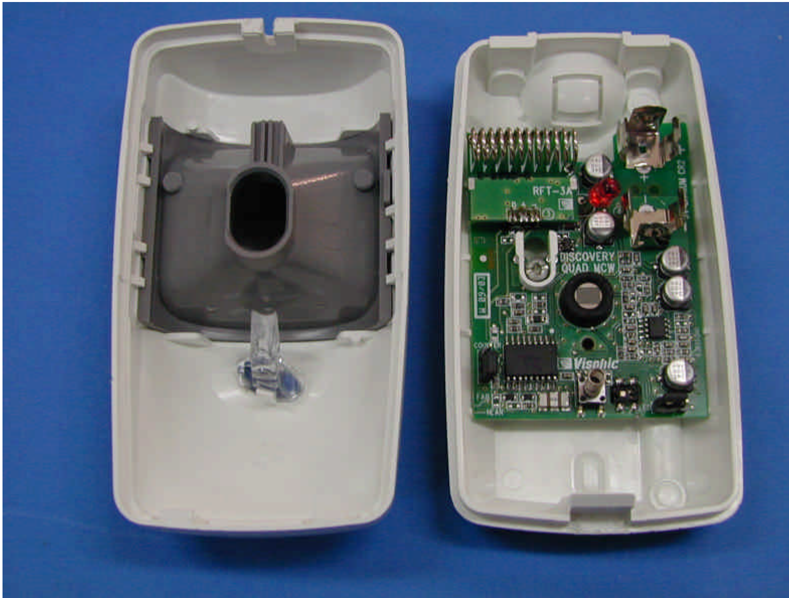
Internal view
