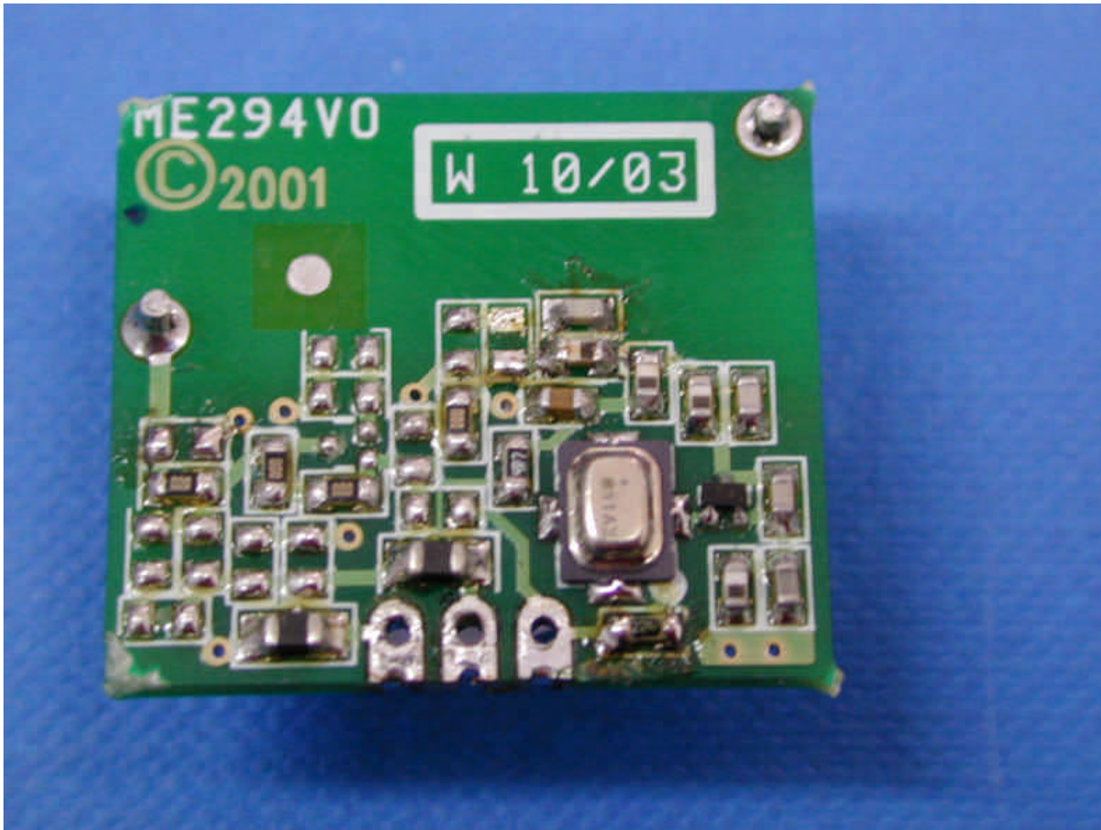
RF module second side
