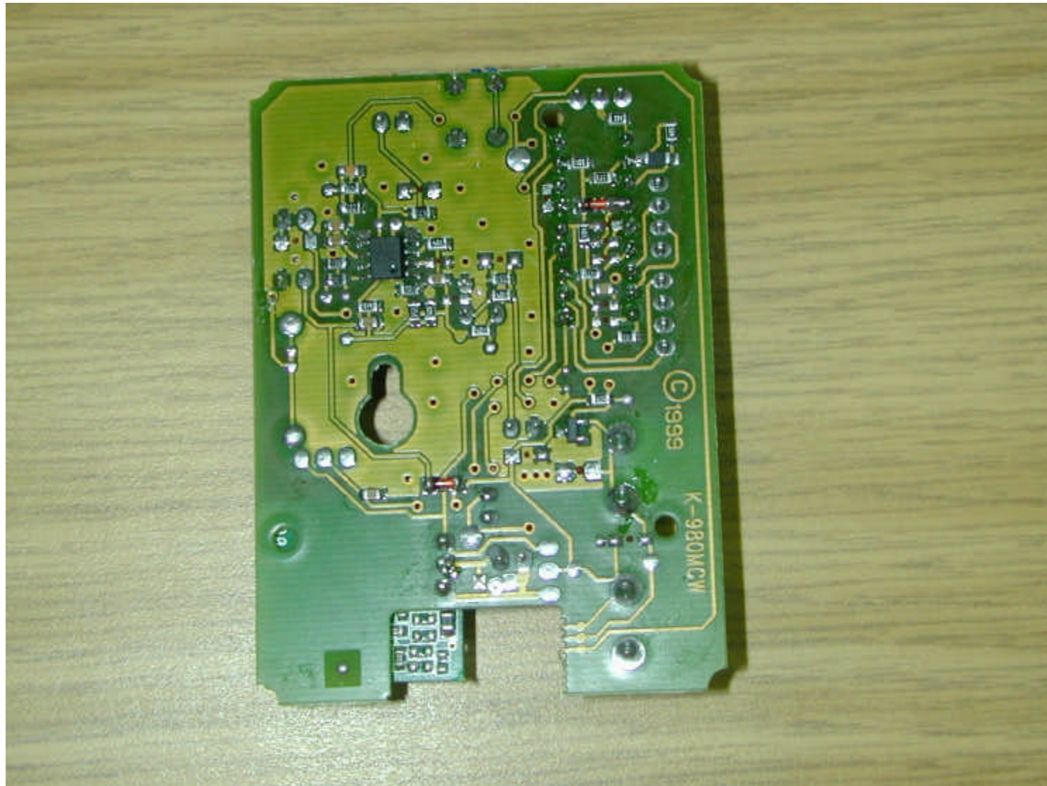
PCB print side
