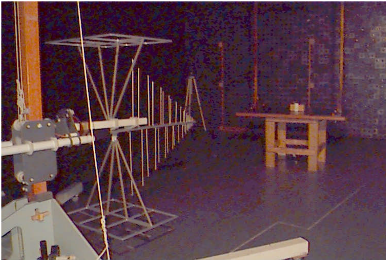
Test setup with log-periodic antenna
