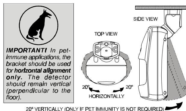
Figure 7. Tilt/Swivel Limits
