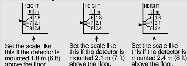
Figure 9. Vertical Adjustment
