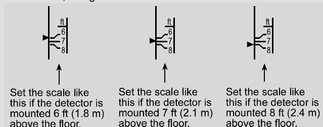
Figure 11. Vertical Adjustment
