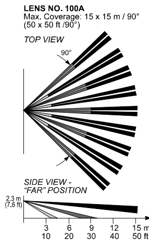
Figure 2. Coverage Pattern
