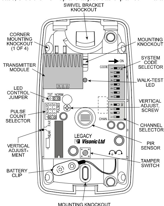
Figure 4. Inside View
