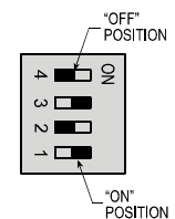
Figure 9. Channel Code Selector
