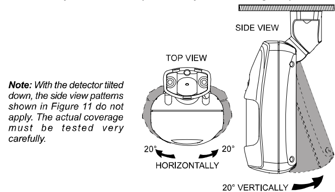
Figure 7. Tilt / Swivel Limits
