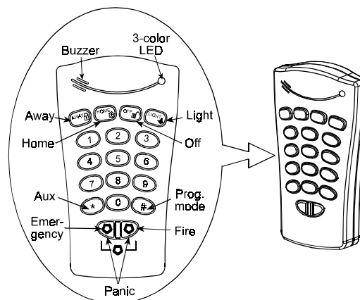
Figure 1 - External View
