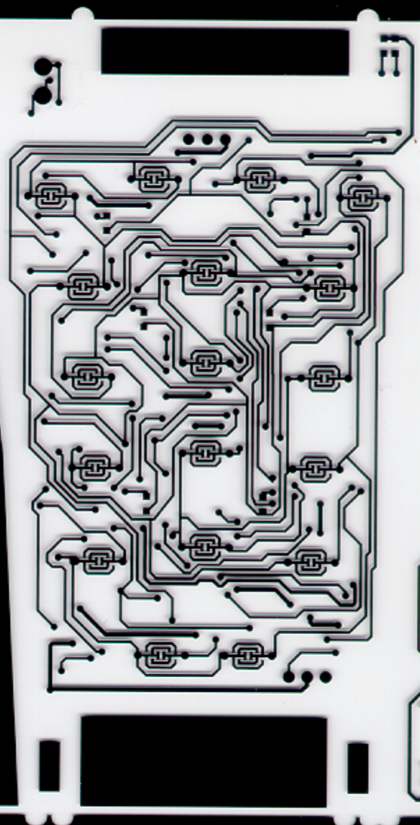
KEYPAD 03 PCB LAYOUT-SOLDER SIDE
