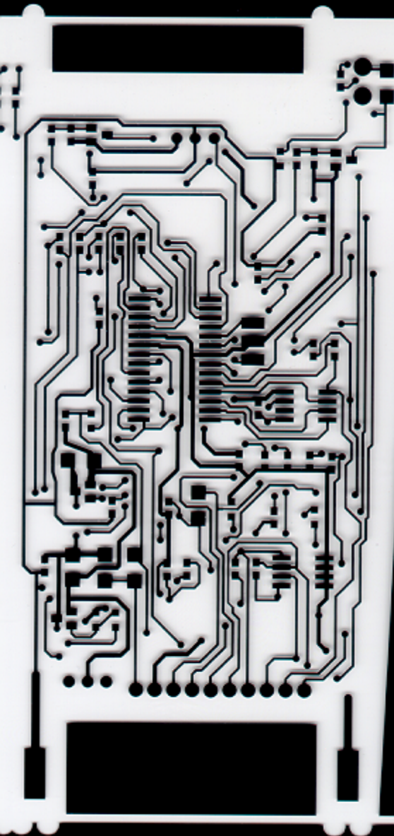
KEYPAD 03 PCB LAYOUT-COMPONENT SIDE
