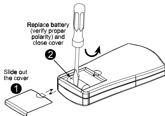
Figure 3 - Battery Replacement
