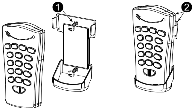
Figure 2 - Mounting
