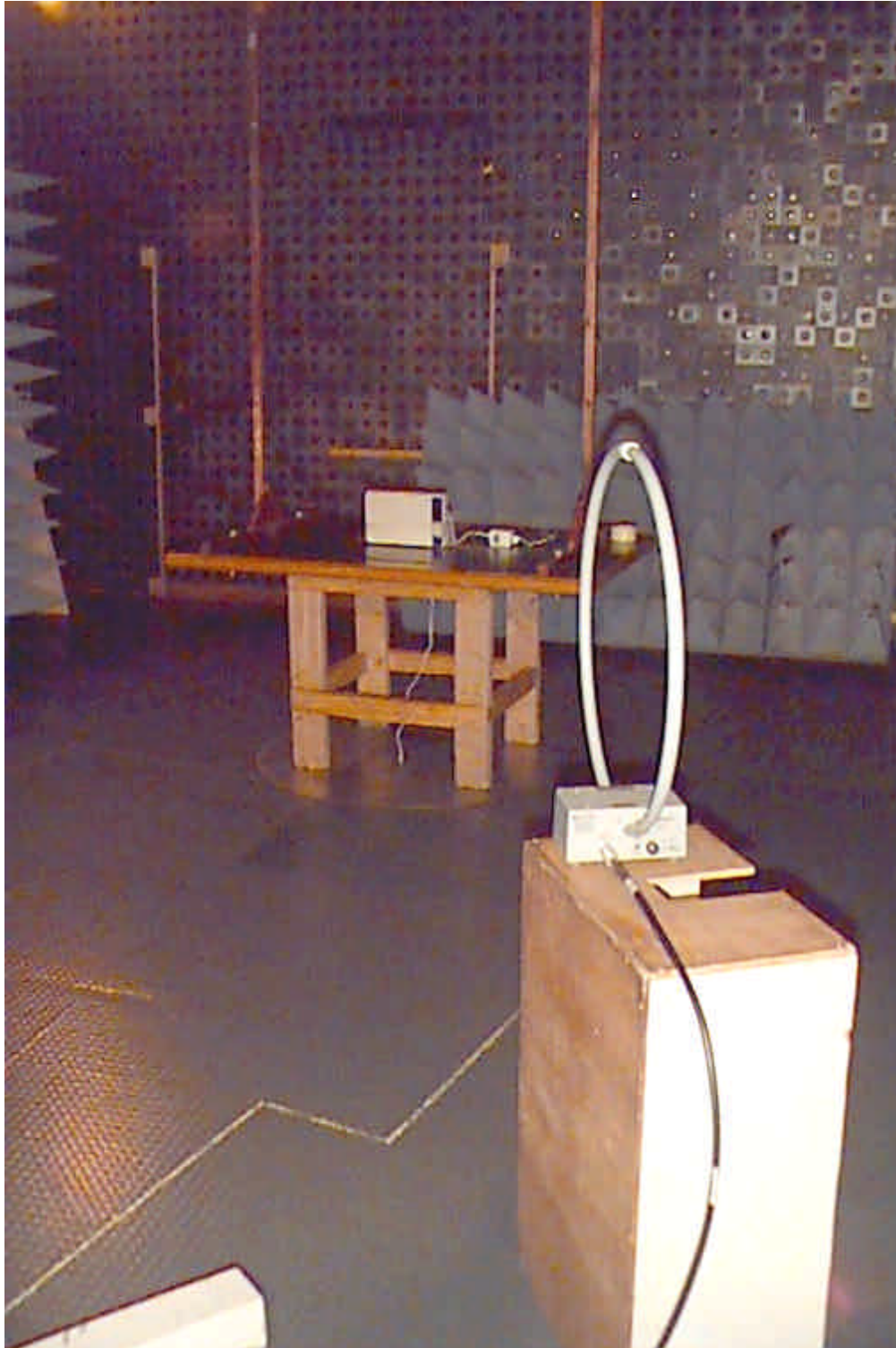
Photograph No.1 Spurious radiated emissions measurement setup in the anechoic chamber with loop antenna
