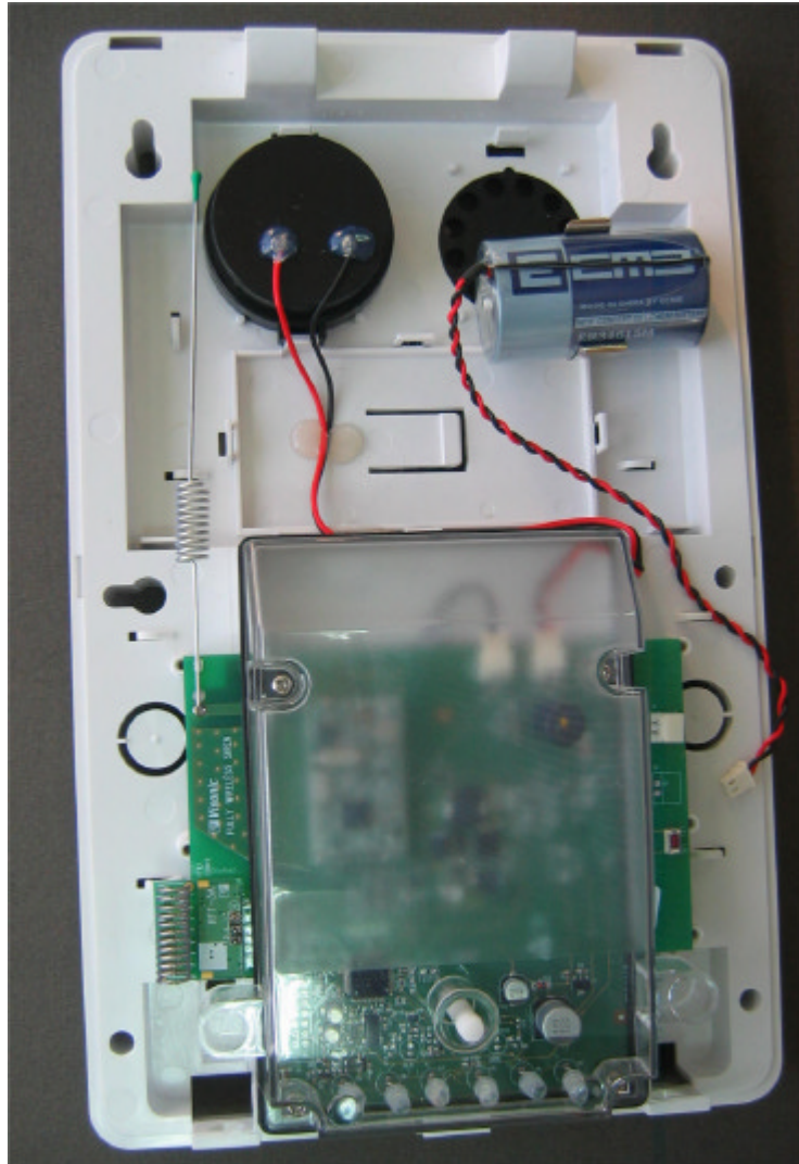
Photograph No2 MCS710 wireless siren internal view
