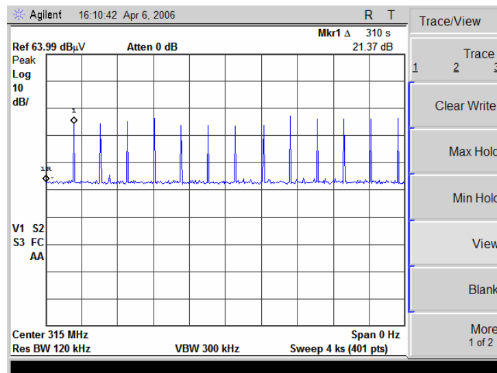
Plot 7.1.2 Polling / supervision transmission duration in 1 hour
