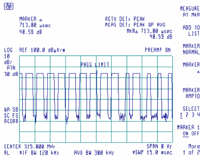
Plot 7.2.12 Transmission pulse period
