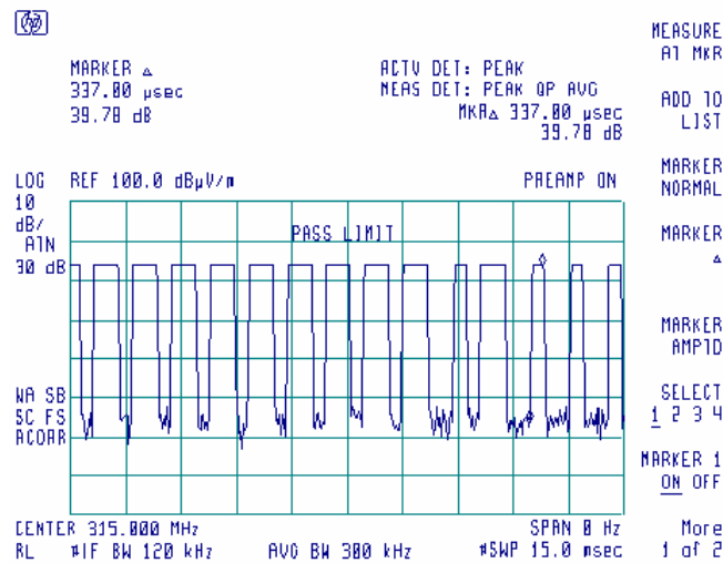
Plot 7.2.10 Transmission pulse period
