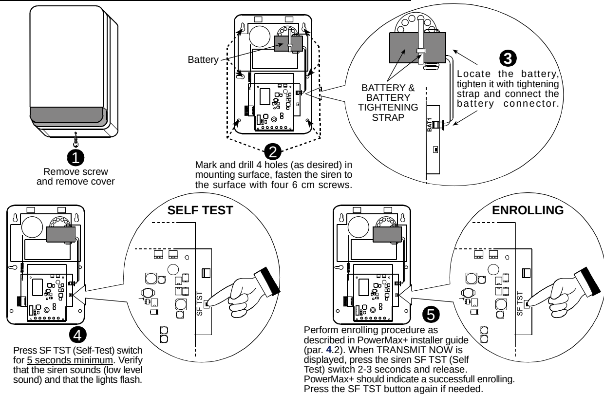
Figure 3 – Installation, Testing and Enrolling
