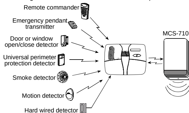
Figure 2- Integration with the Alarm System
