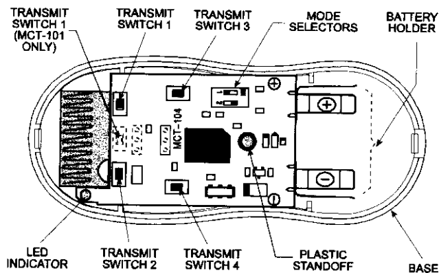
Figure 3. Component Layout
