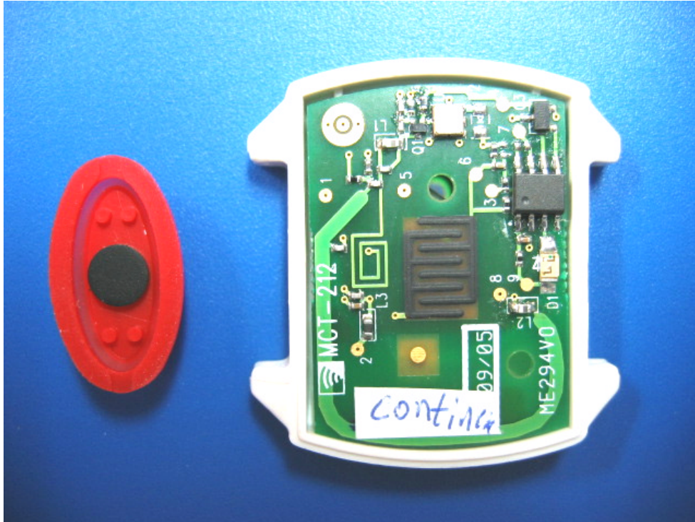
Photograph No.2 Wrist transmitter, model MCT-212RL Internal view
