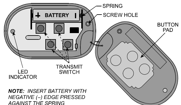
Figure 2. Inside View with Cover Removed
