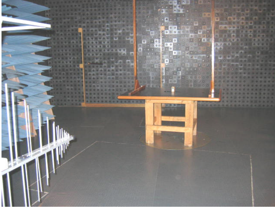
Photograph No.5 Setup for unintentional radiated emission measurements in anechoic chamber from 30 to 1000 MHz
