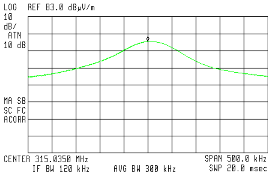
Figure 12. Field Strength of Fundamental. Antenna Polarization: HORIZONTAL. Detector: Peak
