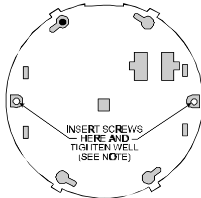
Figure 7. Securing the Cover to the Base
