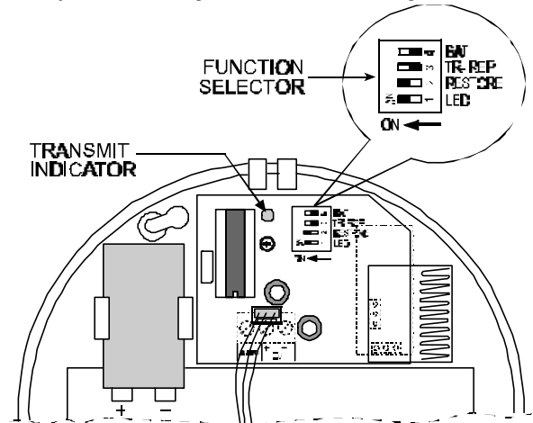
Figure 3. Transmit Indicator and Function Switch
