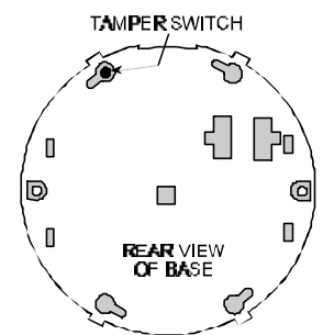
Figure 4. Tamper Switch
