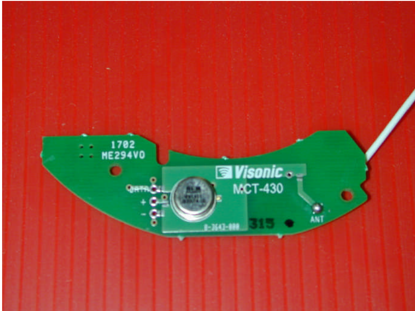
Small PCB second side
