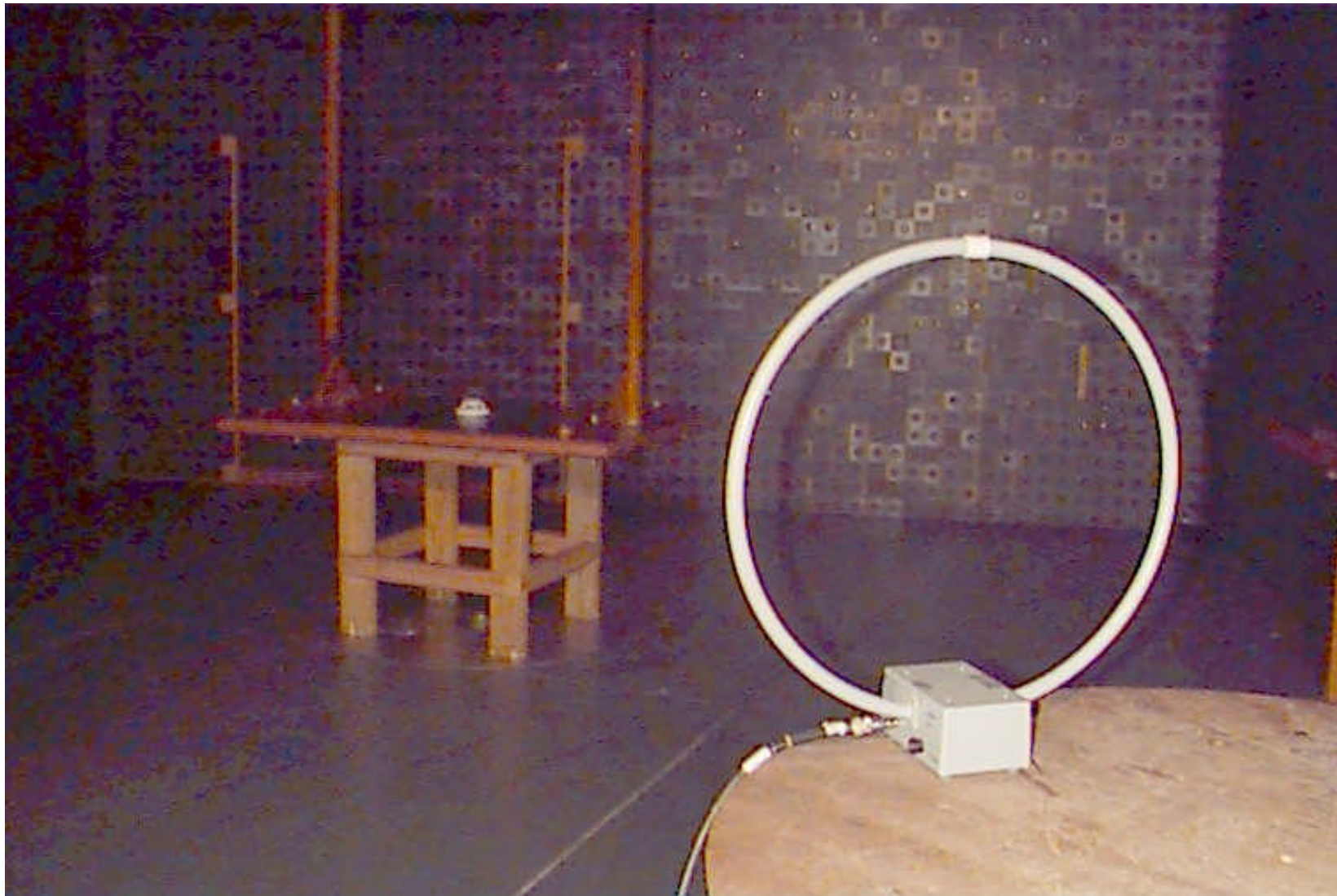
Test setup with loop antenna
