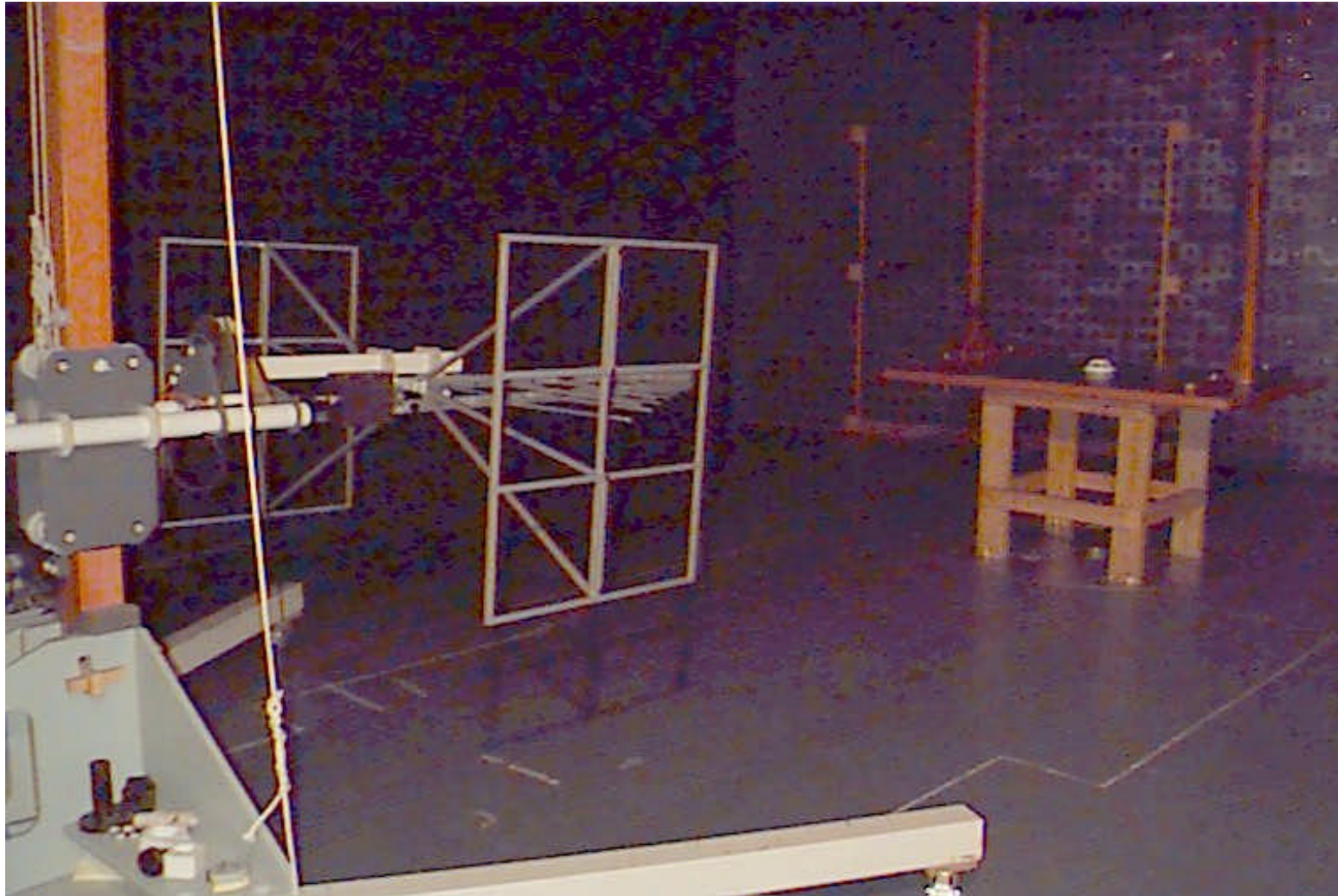
Test setup with biconical antenna
