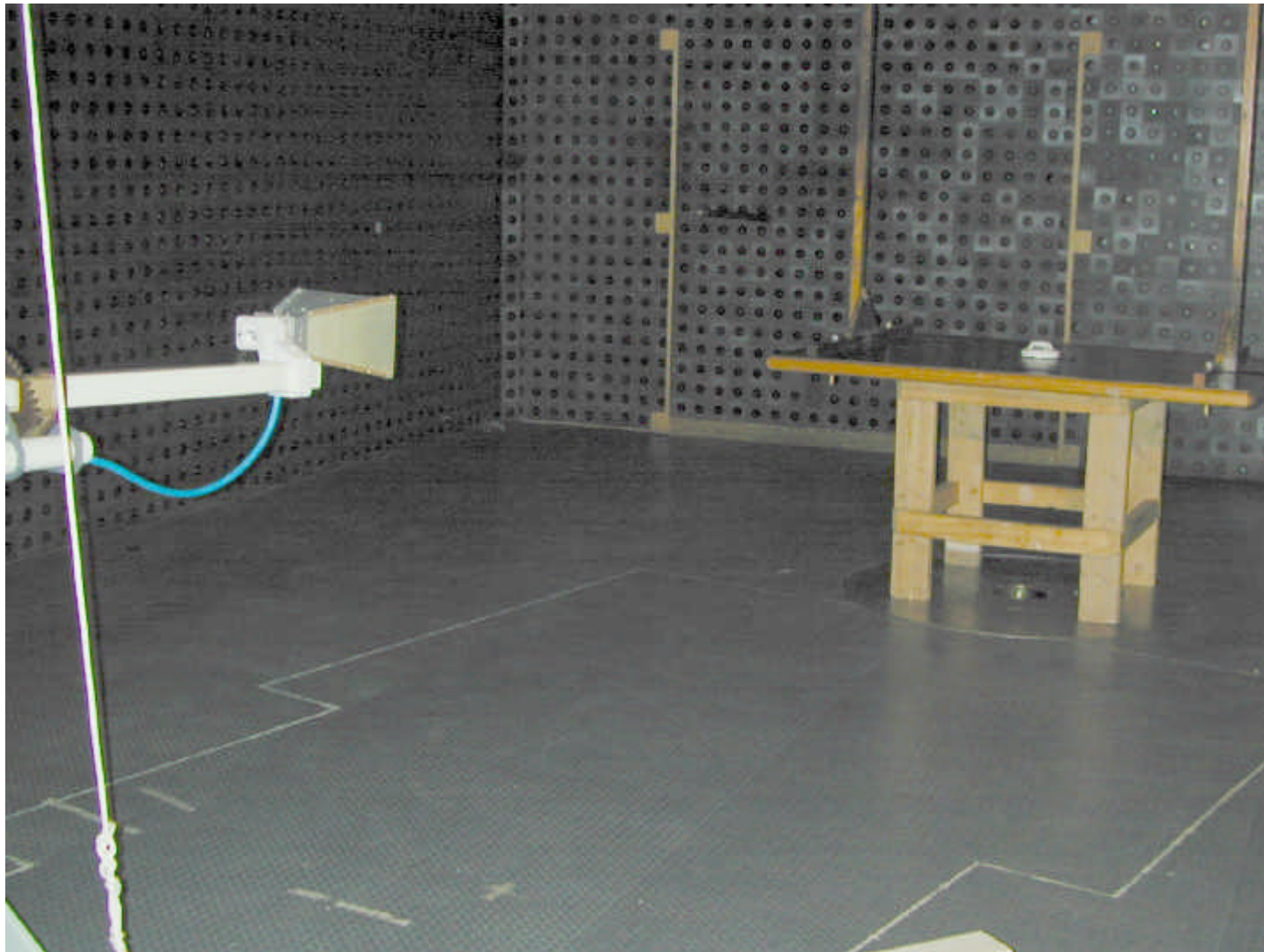
Test setup with double ridged guide antenna
