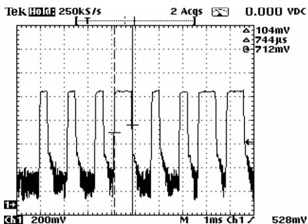
Plot 7.2.13 Transmission pulse duration (BIT 1)
