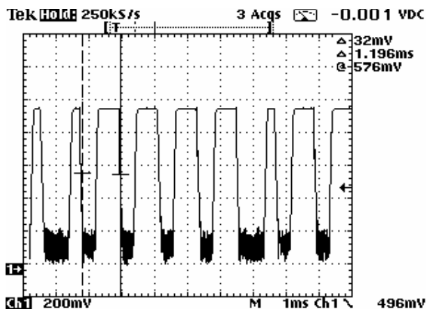
Plot 7.2.14 Transmission pulse period (BIT 1)
