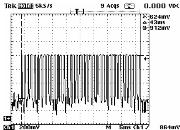
Plot 7.2.12 Transmission burst period
