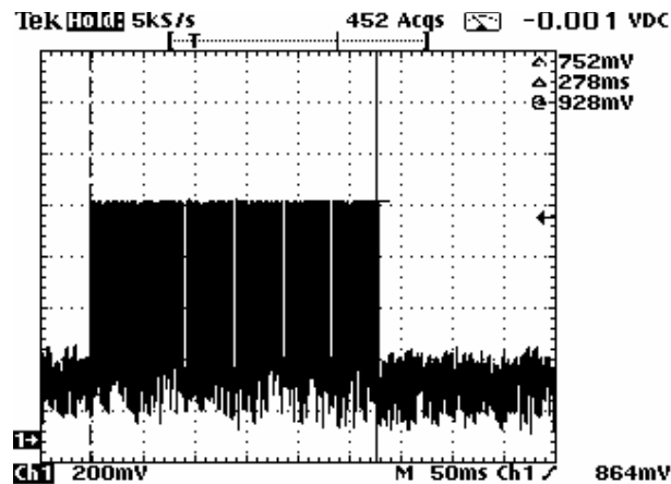
Plot 7.2.9 Transmission train duration
