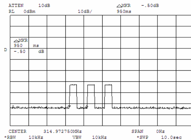
Plot 7.1.3 Transmitter supervision duration test result
