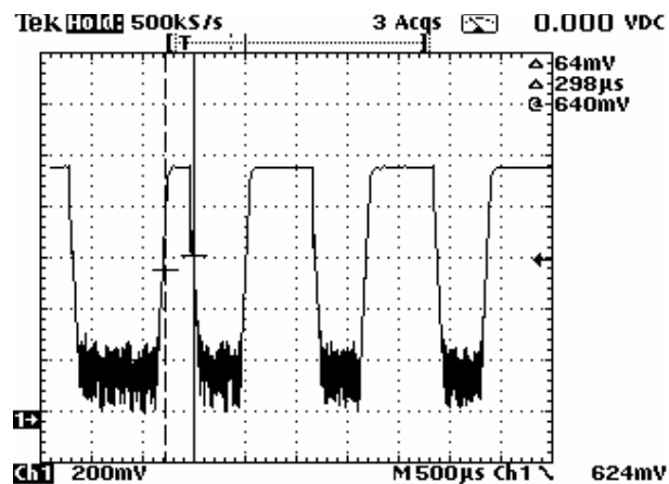
Plot 7.2.15 Transmission pulse duration (BIT 0)
