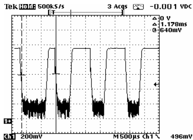
Plot 7.2.16 Transmission pulse period (BIT 0)
