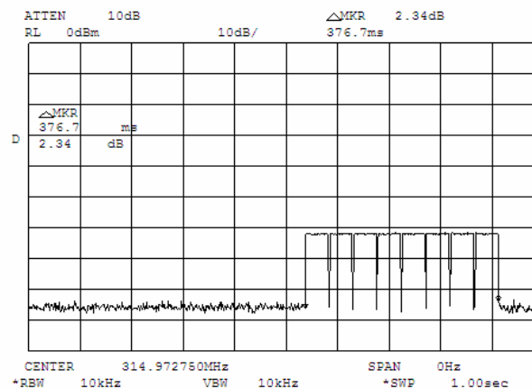
Plot 7.2.10 Transmission supervision train duration
