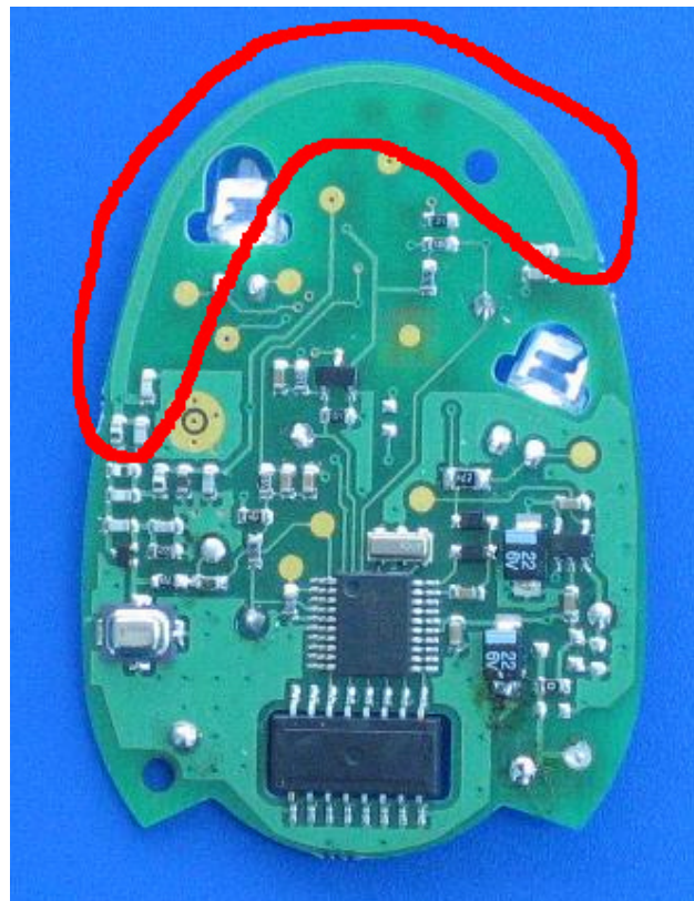
Photograph 7.4.1 Antenna assembly
