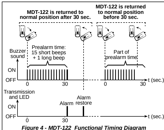
Figure 4 - MDT-122 Functional Timing Diagram
