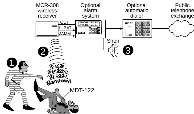
Figure 1 - Integration of MDT-122 in an Alarm System
