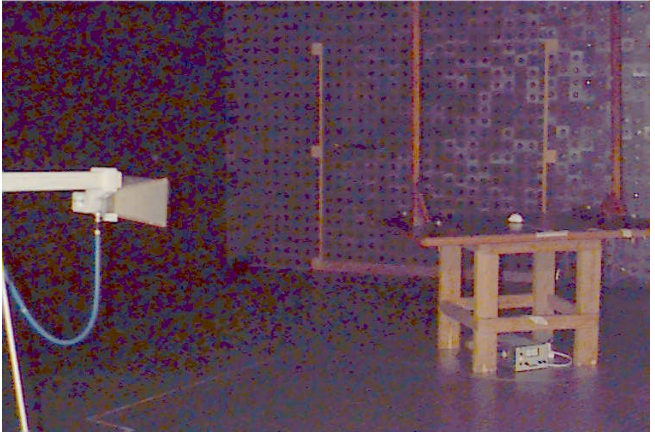
Photograph 3 Test setup with double ridged guide antenna (2 to 18 GHz frequency range)
