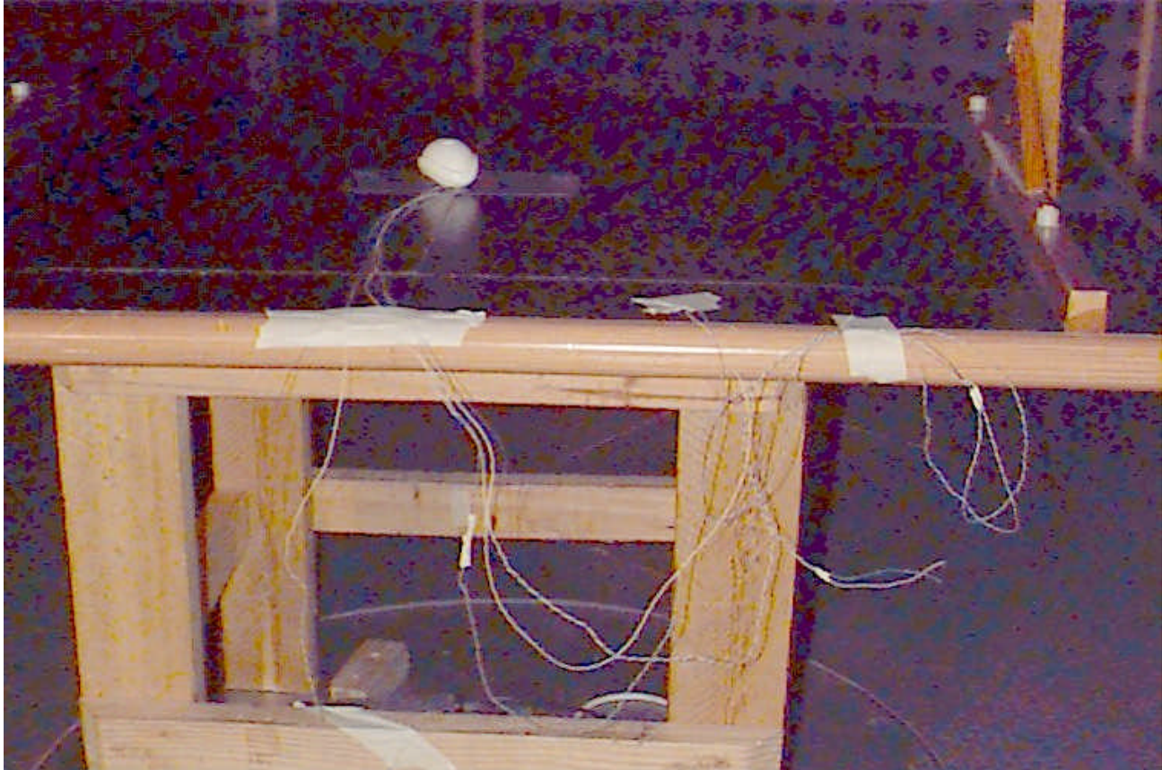
Photograph 5 EUT position during the testing
