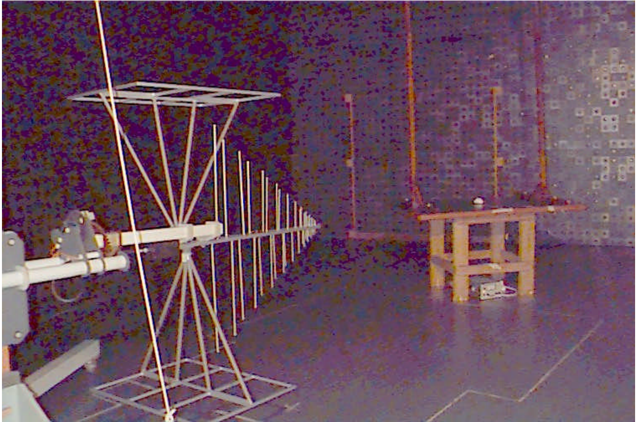
Photograph 2 Test setup with biconilog antenna (30 to 2000 MHz frequency range)
