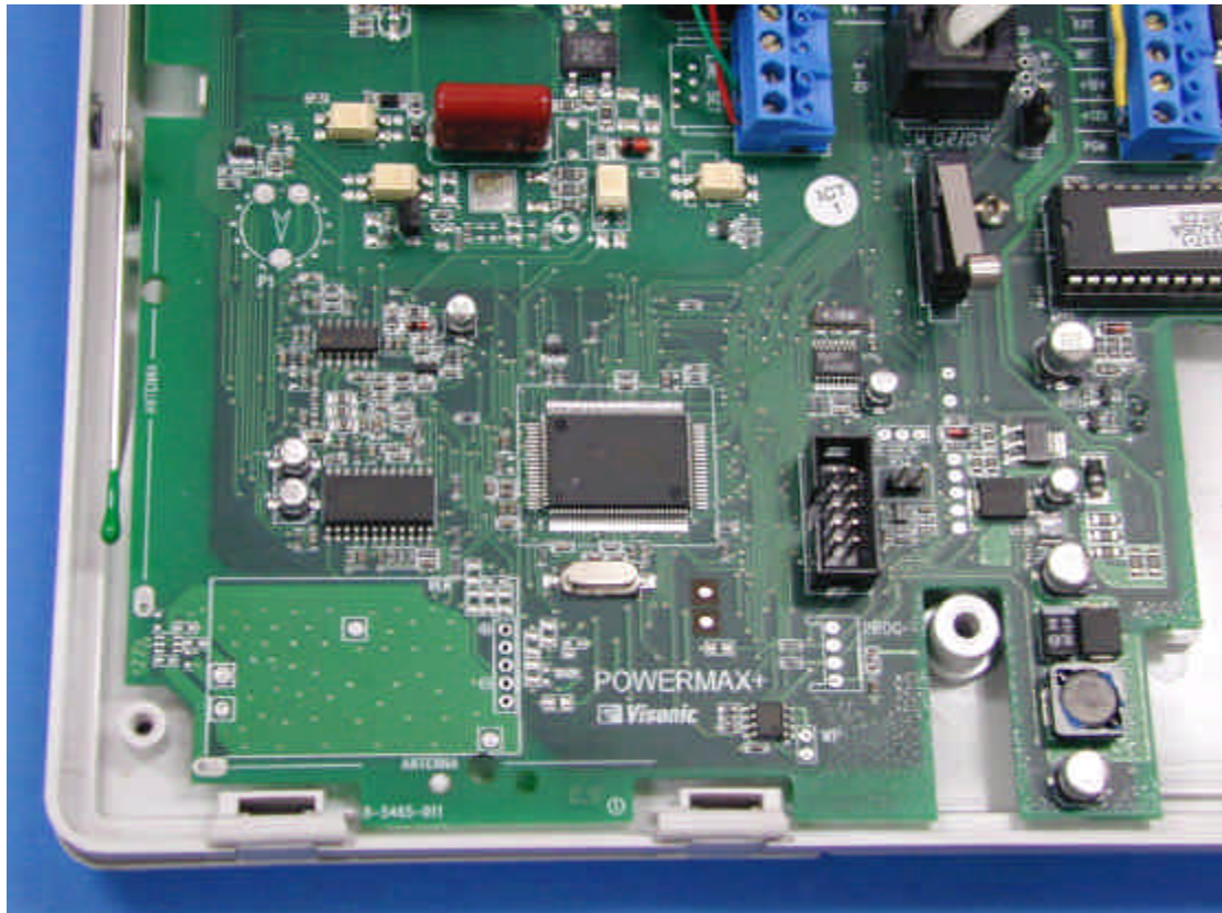
Photograph No.3 POWERMAX+ alarm control panel Internal view, left low part
