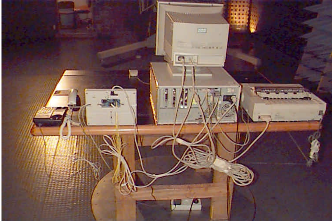
Photograph No.5 Radiated emissions measurement setup in the anechoic chamber
