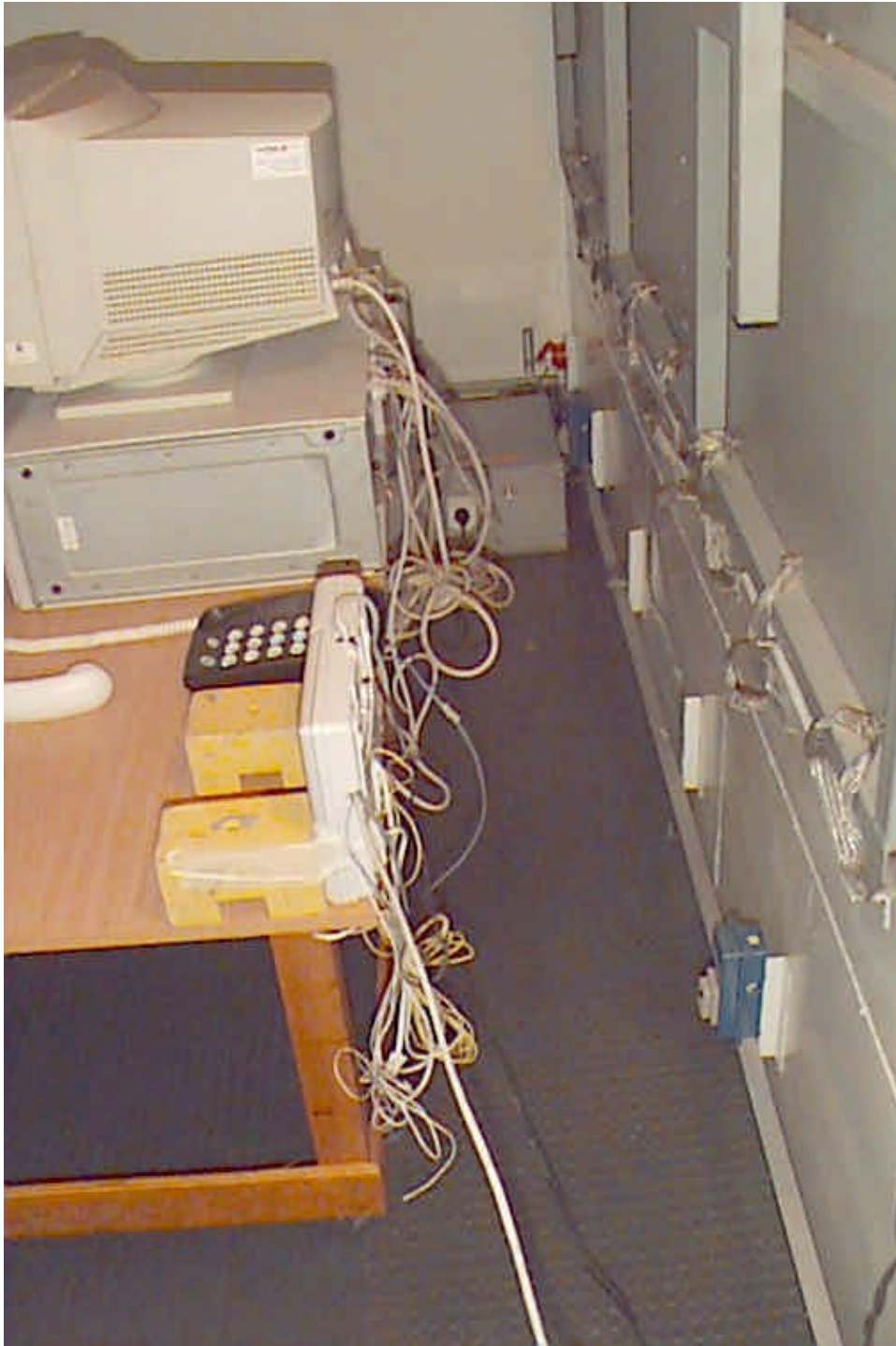
Photograph No.7 Conducted emissions measurement setup on EUT power ports
