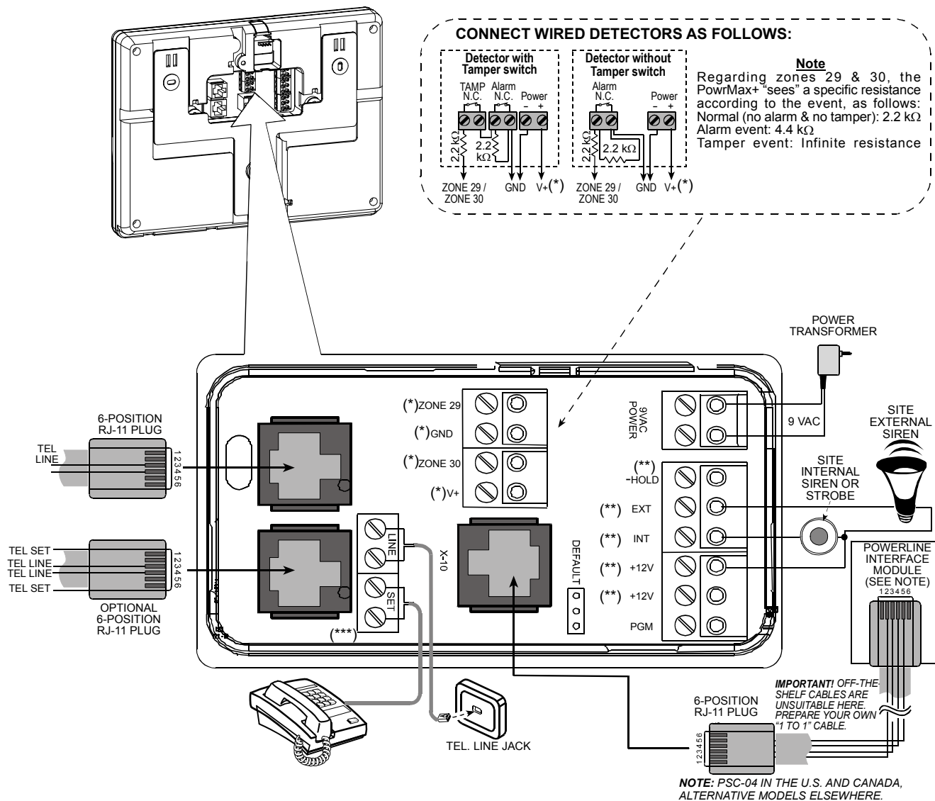
Figure 3 - Wiring Diagram
