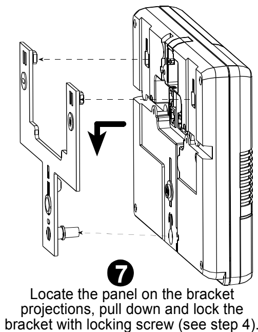
Figure 2 - Mounting
