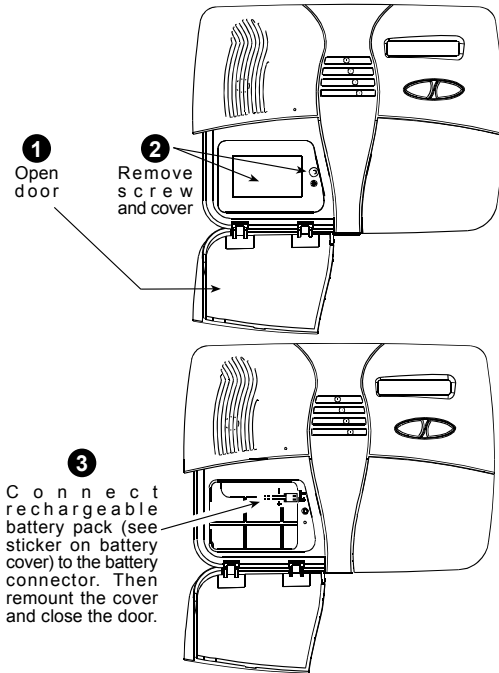
Figure 10. Battery Replacement
