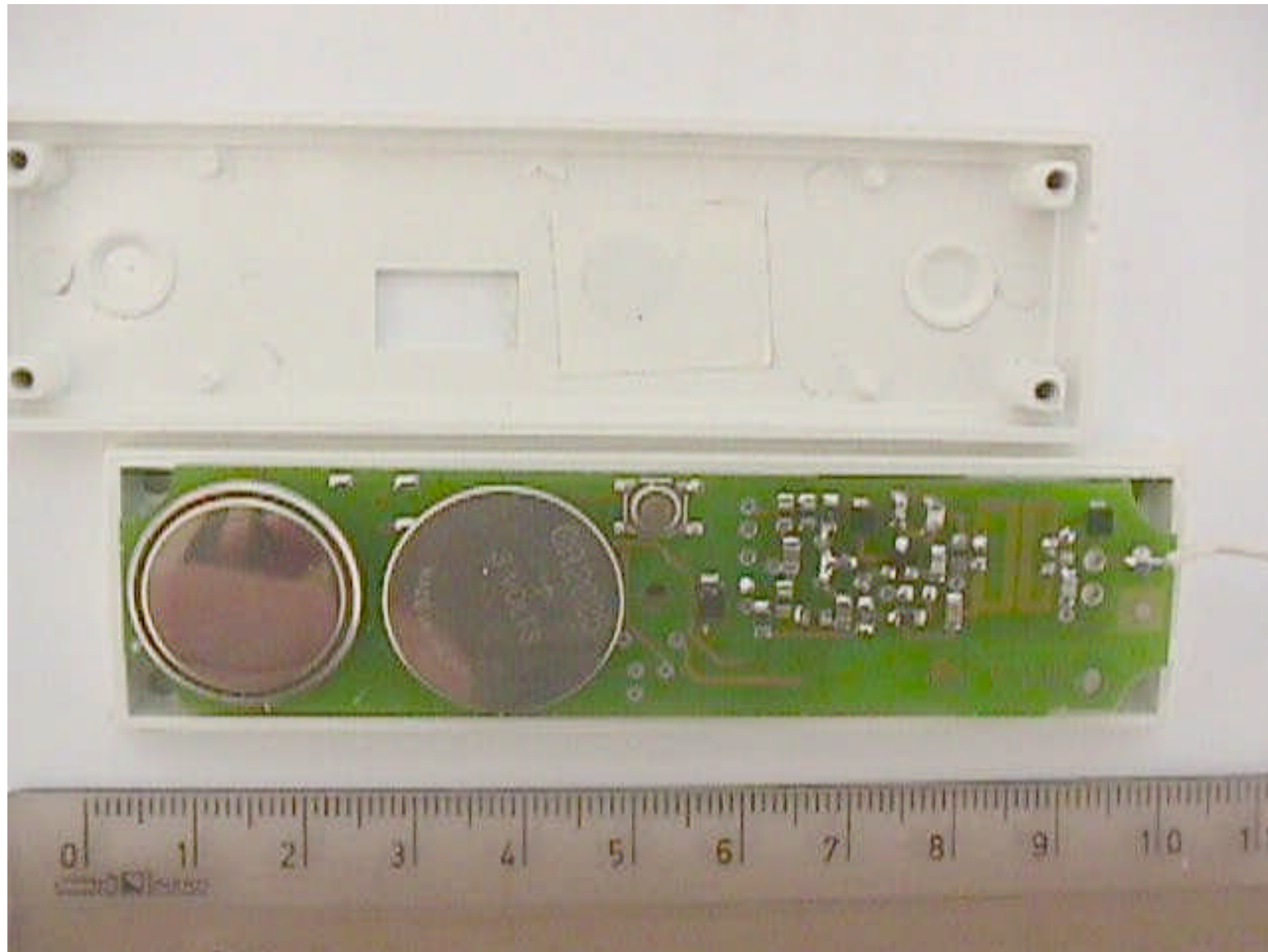
SPD-1000 internal view (second side)
