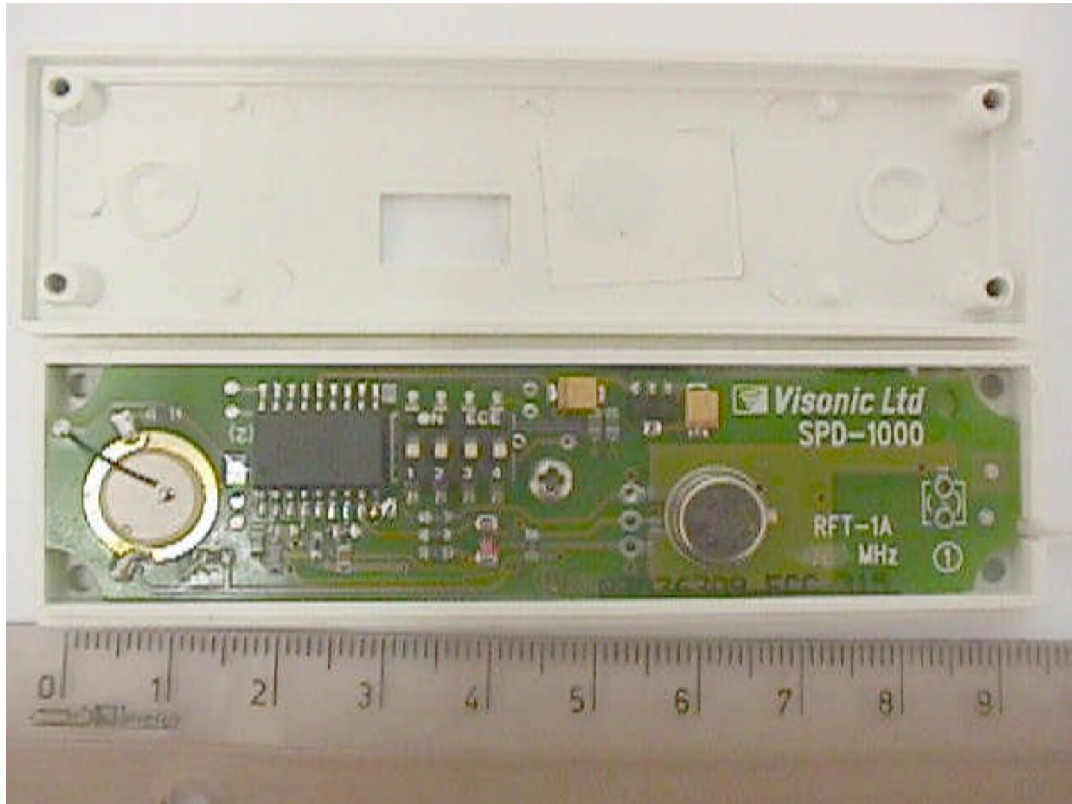
SPD-1000 internal view (first side)
