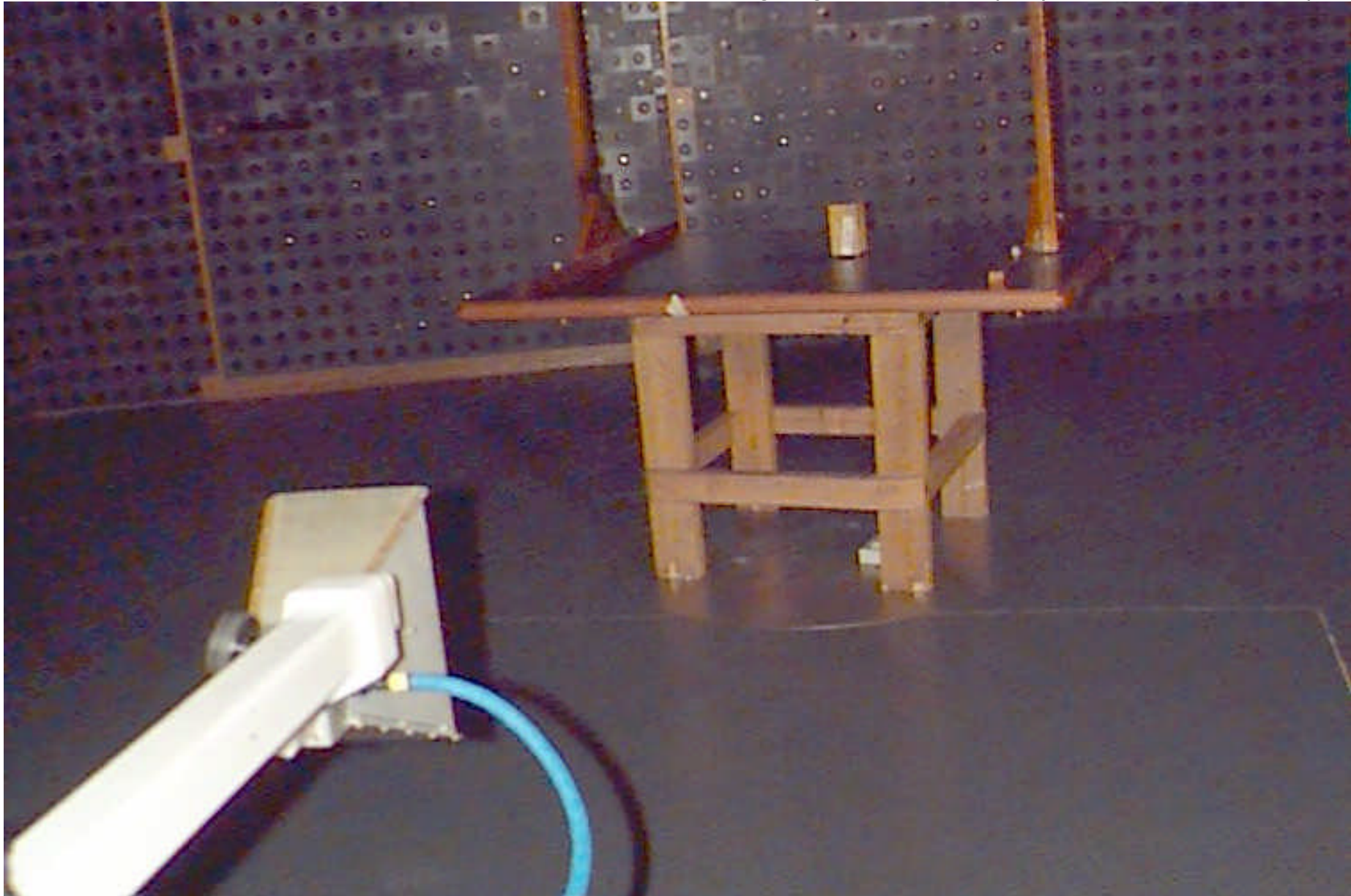
Unintentional radiated emission measurements with double ridged guide antenna (frequencies above 1 GHz)
