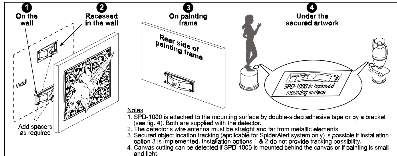
Figure 3 - Installation Possibilities
