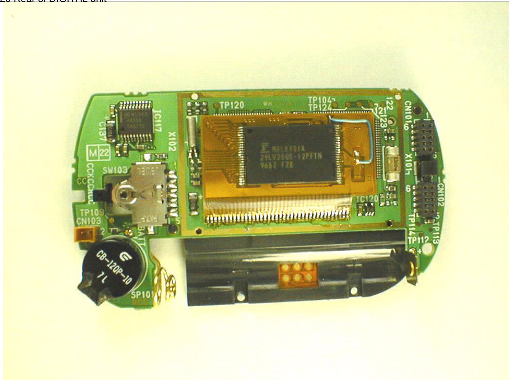
PB2320 Rear of DIGITAL unit
