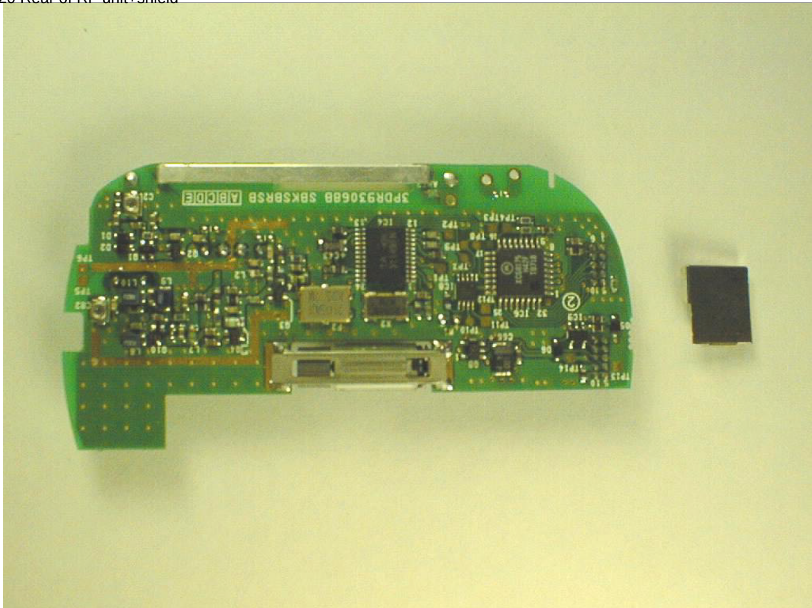
PB2320 Rear of RF unit+shield
