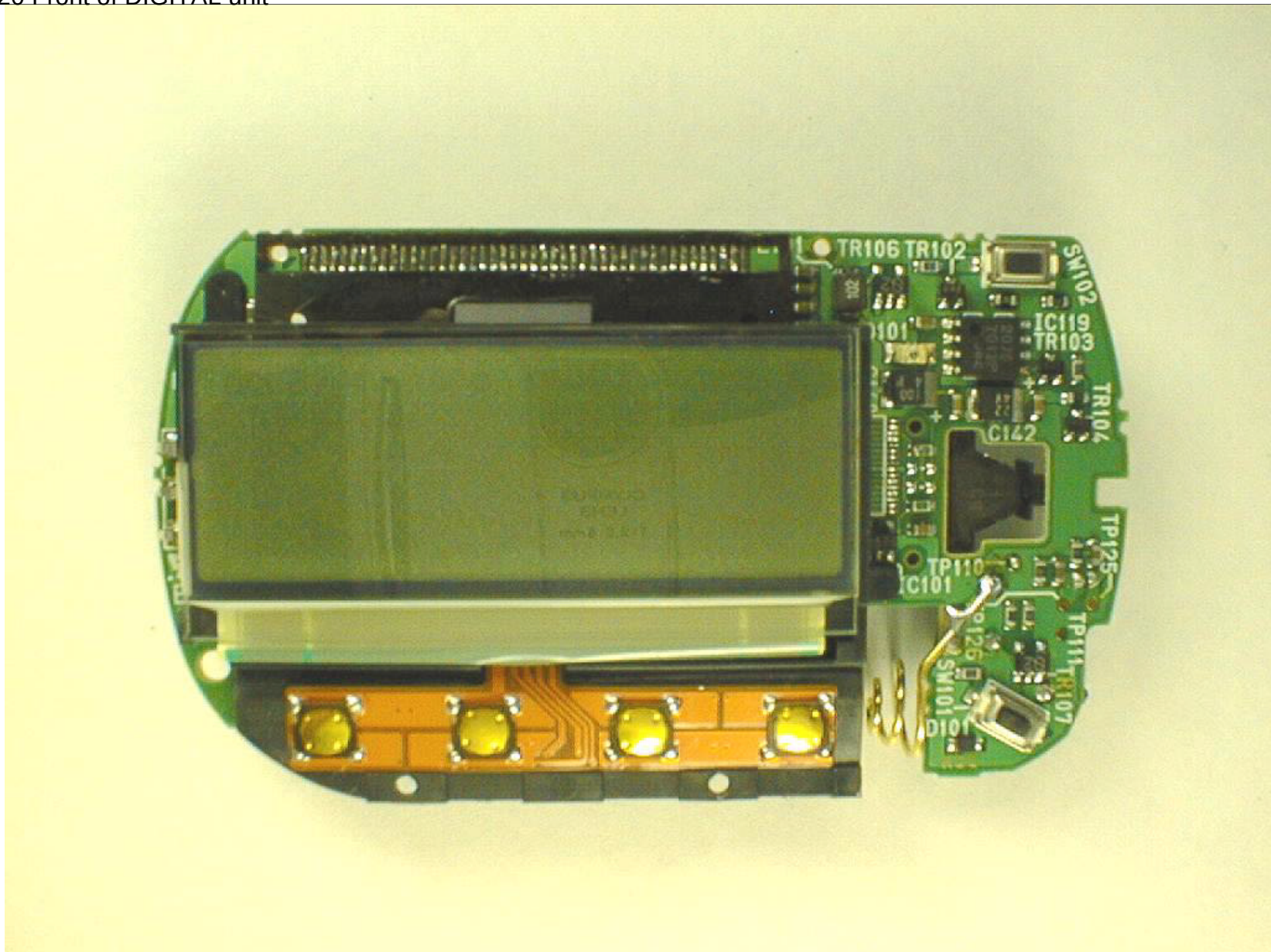
PB2320 Front of DIGITAL unit
