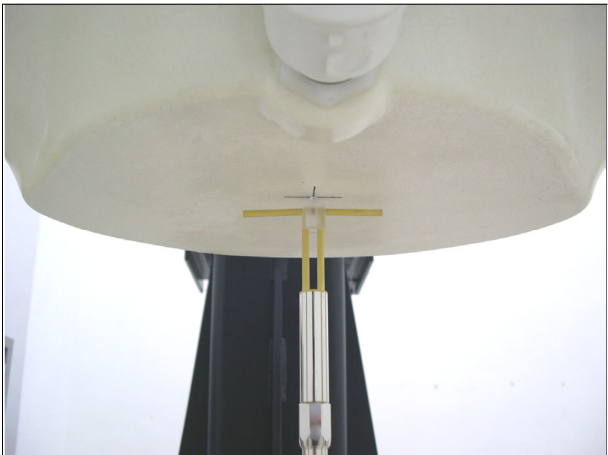
Fig 8.2 Dipole Setup
