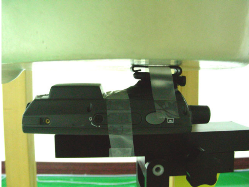
Fig. 9.1 EUT with Belt Clip Touch
