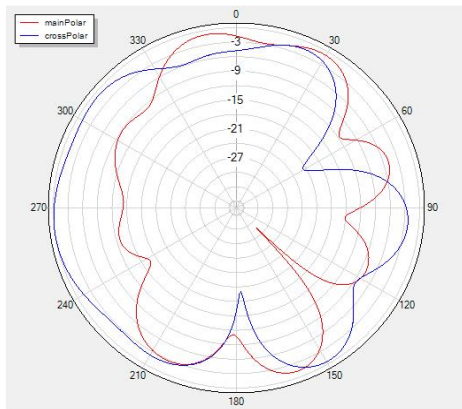
Phi=90 freq=5900MHz
