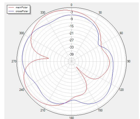
Theta=90 freq=2480MHz
