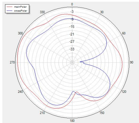
Phi=0 freq=5900MHz
