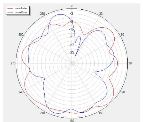
Theta=90 freq=2480MHz
