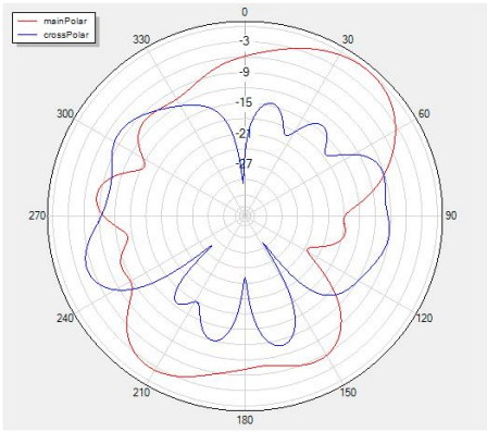
Phi=90 freq=5650MHz
