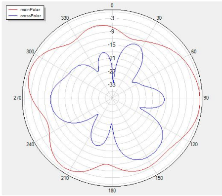
Phi=0 freq=5650MHz
