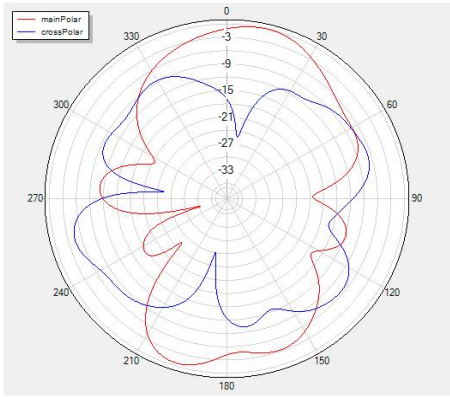
Theta=90 freq=5650MHz
