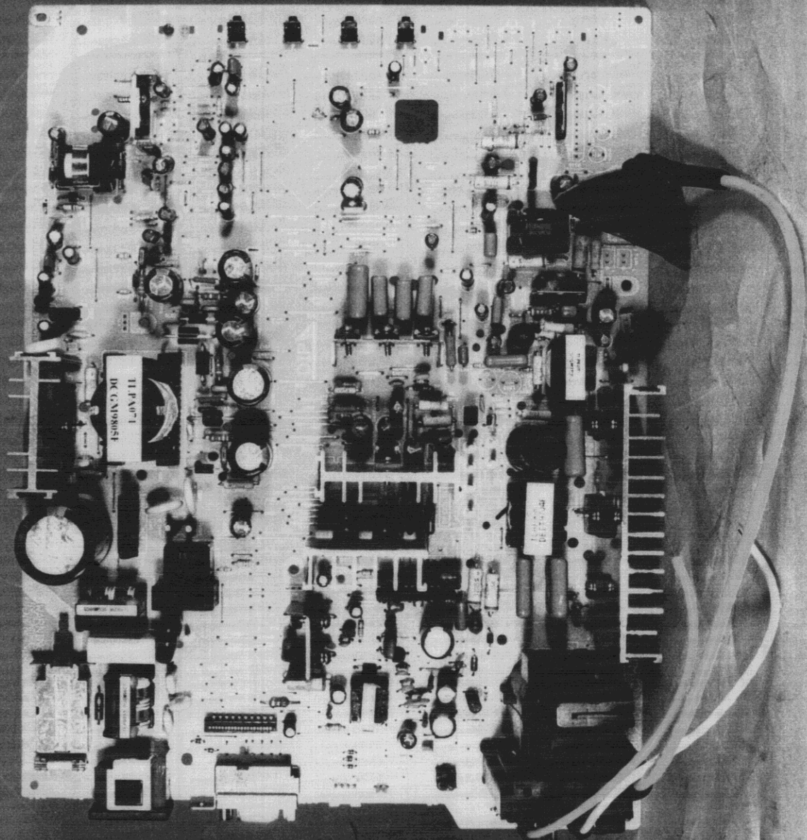
Photo. 4. Main & Power Supply PWB of Model VCDTS21406-2*
