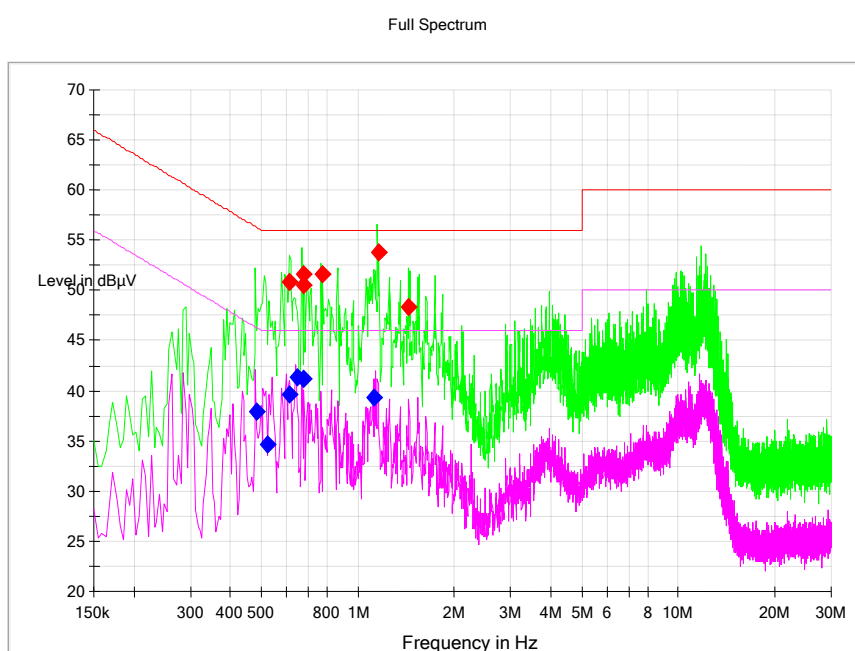
L+N Line
