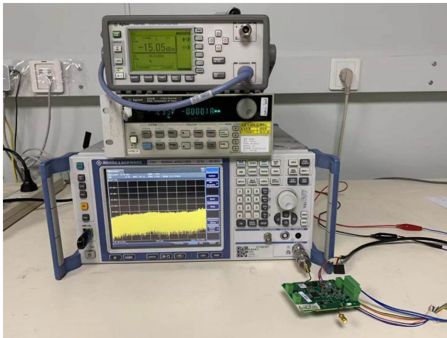
RF Conducted Test setup (BT/ZIGBEE)
