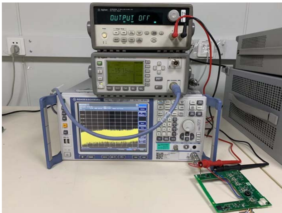
RF Conducted Test setup
