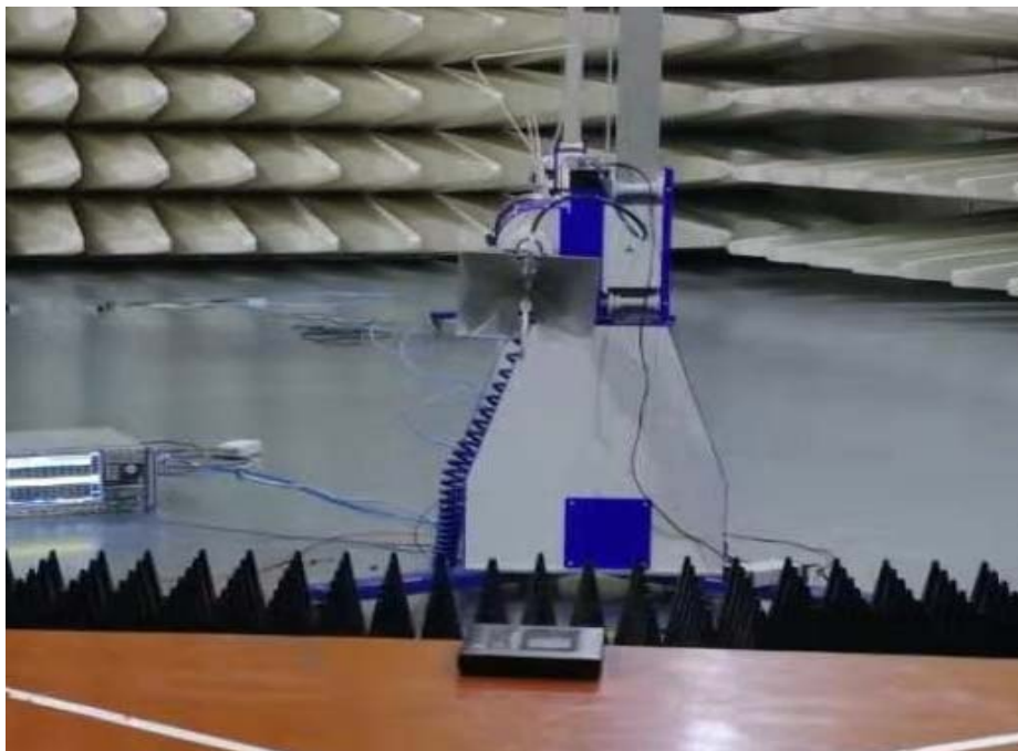
Spurious Radiated Emissions Test setup (1GHz~25GHz)
