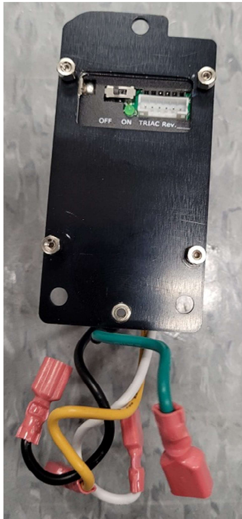
Triac Actuator Front View
