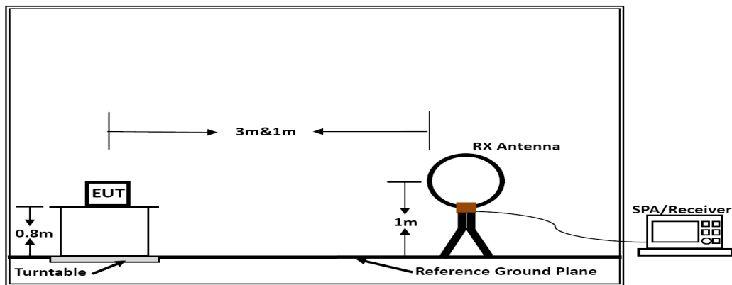
Below 30MHz
