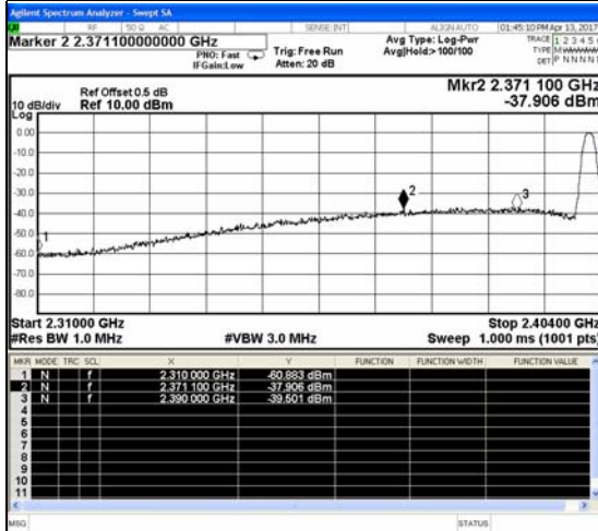
Channel 0 / 2402 MHz – Non-Hopping – Peak
