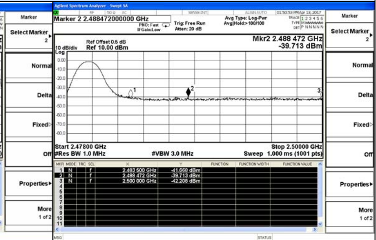
Channel 78 / 2480 MHz – Non-Hopping – Peak
