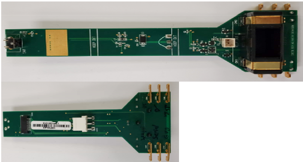
Battery board (no transmitter):
