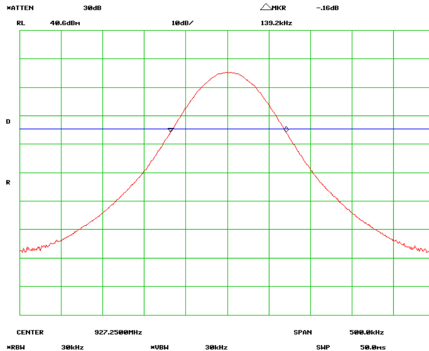
20 dB Bandwidth – High Channel
