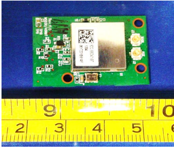
Radio Board – Top View
