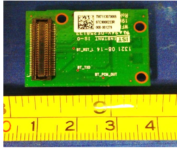
Radio Board – Bottom View
