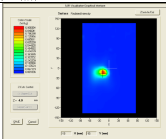
SURFACE SAR
