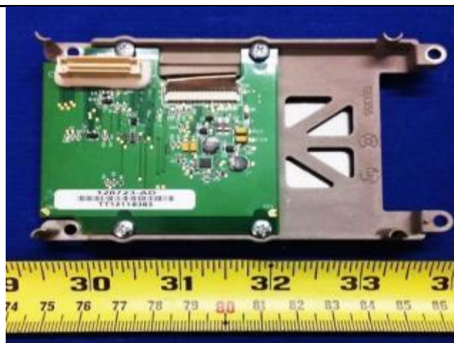
LCD Display - Rear View
