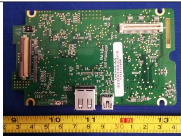
PCBA1 - Front View
