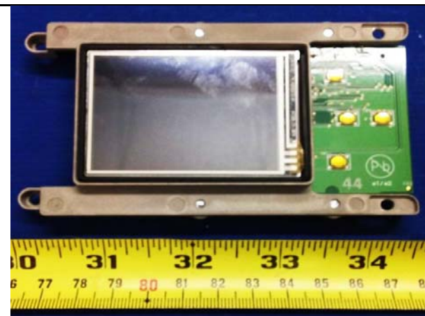
LCD Display - Front View
