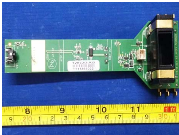
PCBA3 - Front View
