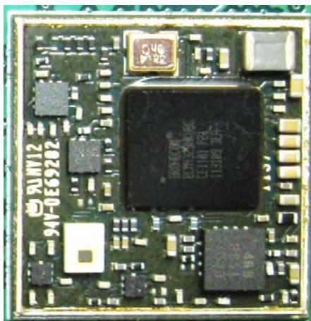
EUT – Top View without shielding
